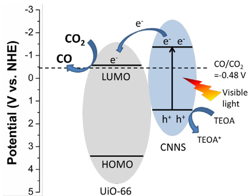
Figure 5. Proposed mechanism of photocatalytic reduction of \text{CO}_2 by \text{UiO-66/CNNS} heterogeneous photocatalyst under visible light irradiation.
